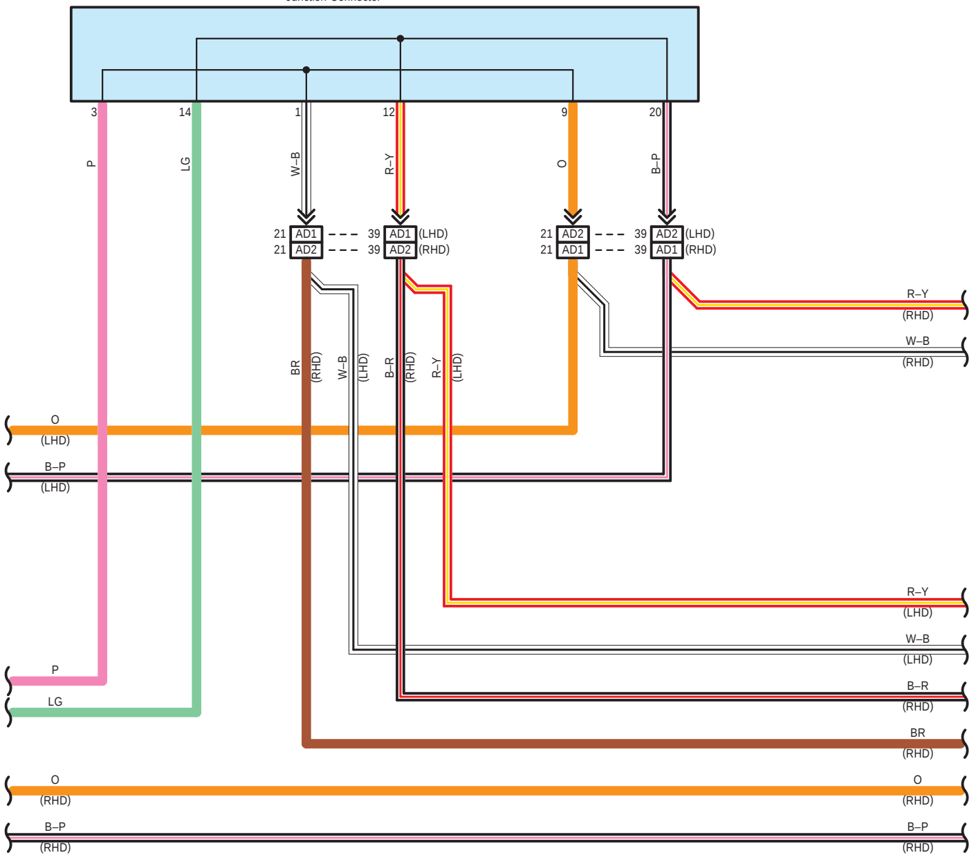
D43 Junction Connector
