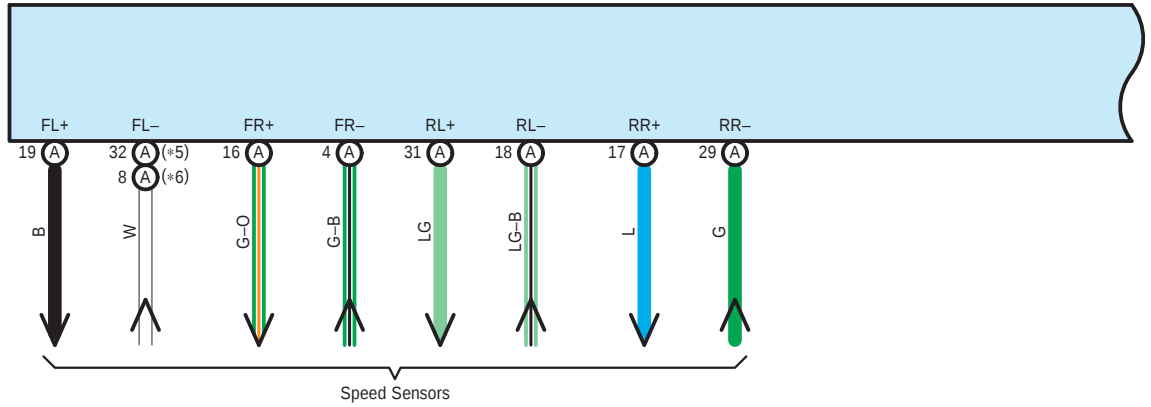
A5(A) Brake Actuator Assembly
