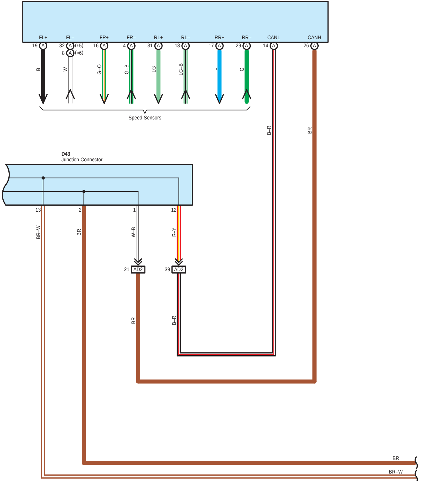
A5(A) Brake Actuator Assembly
