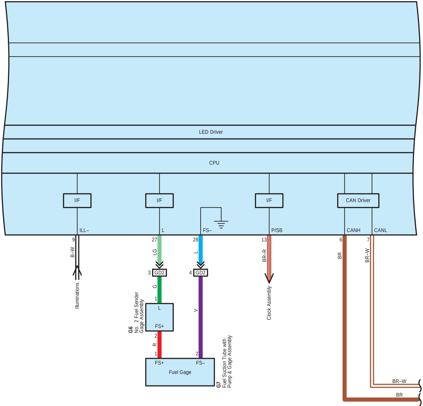
D7 Combination Meter Assembly
