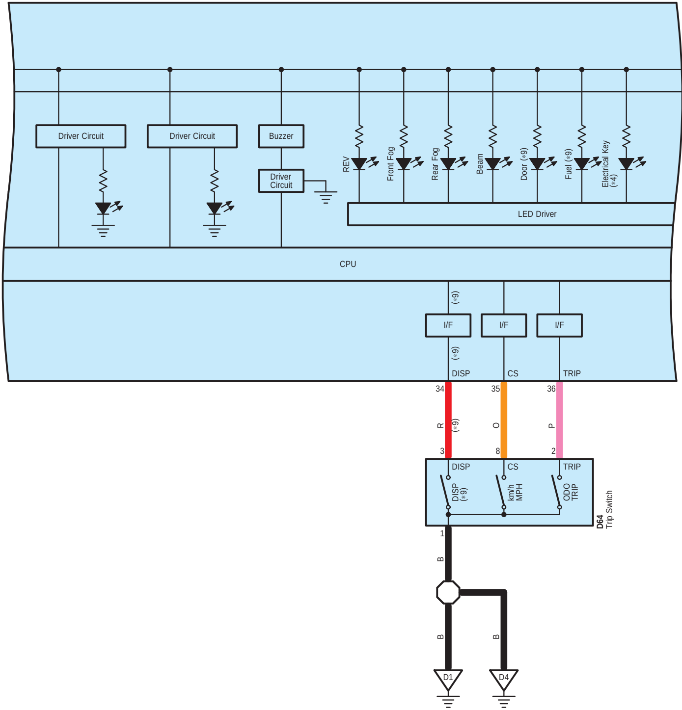
D7 Combination Meter Assembly
