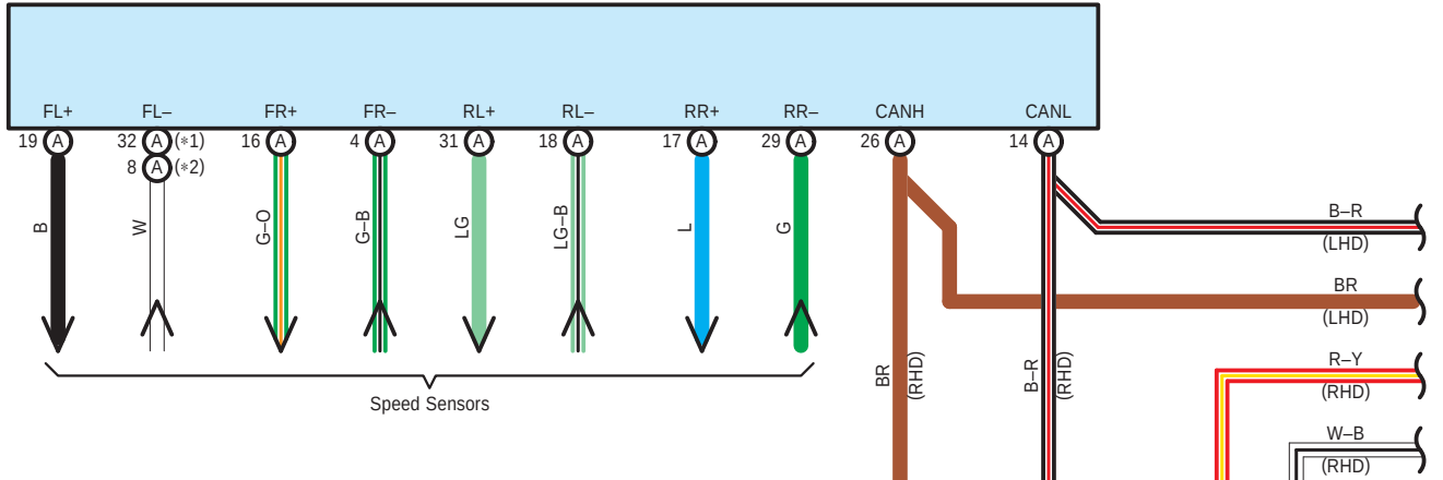
A5(A) Brake Actuator Assembly
