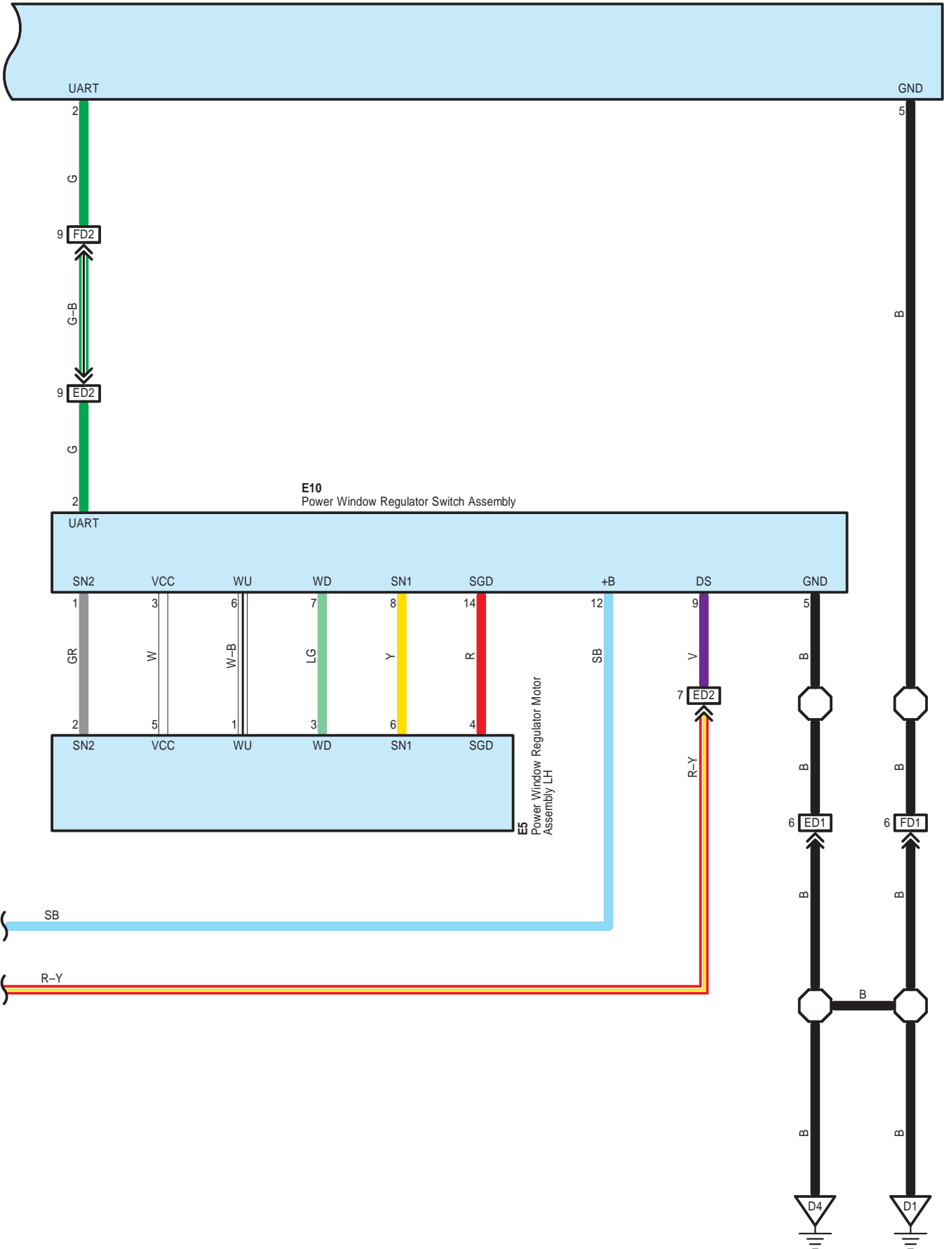
F10 Power Window Regulator Master Switch Assembly
